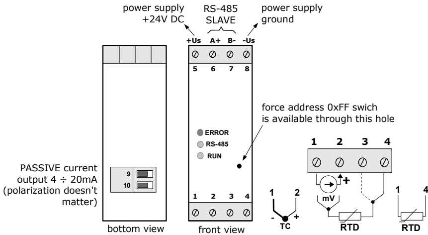
Fig. 4.2. Terminals description
