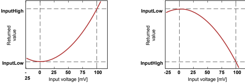
Fig. 6.2 Normal ("InputLow" < "InputHigh") and inverted ("InputLow" > "InputHigh") characteristic.
