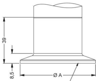
Clamp (DIN 32676)
