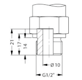
G1/2" open port
